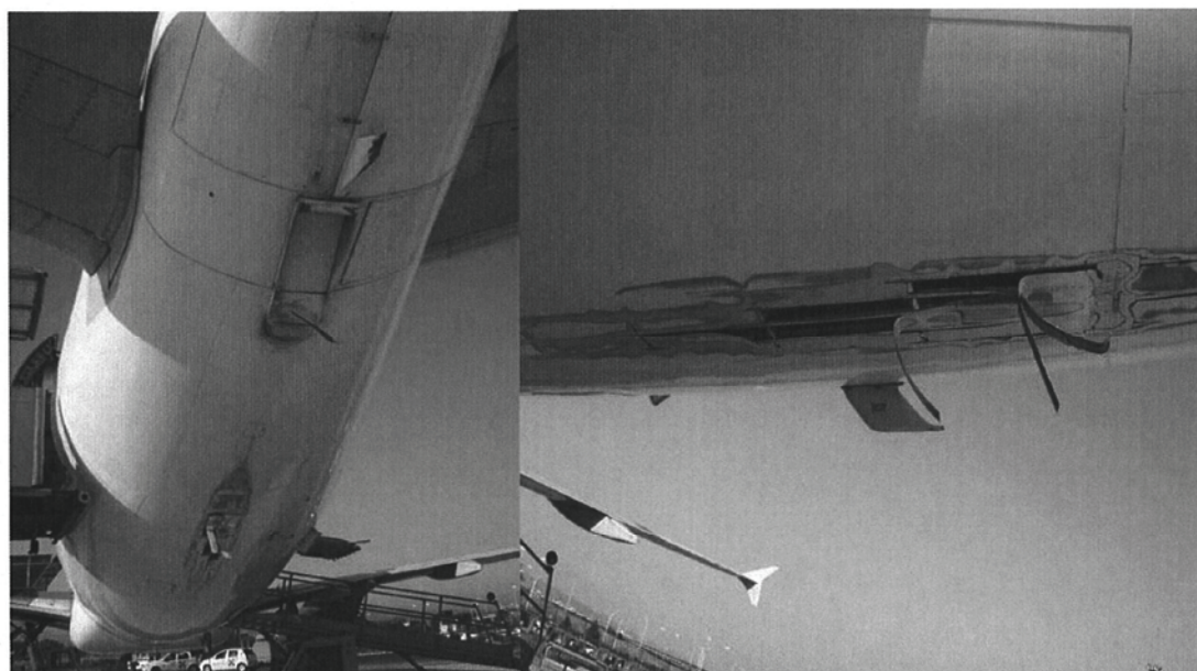
LZ-BHC: extensive structural damages to the lower part of the tail fuselage.
